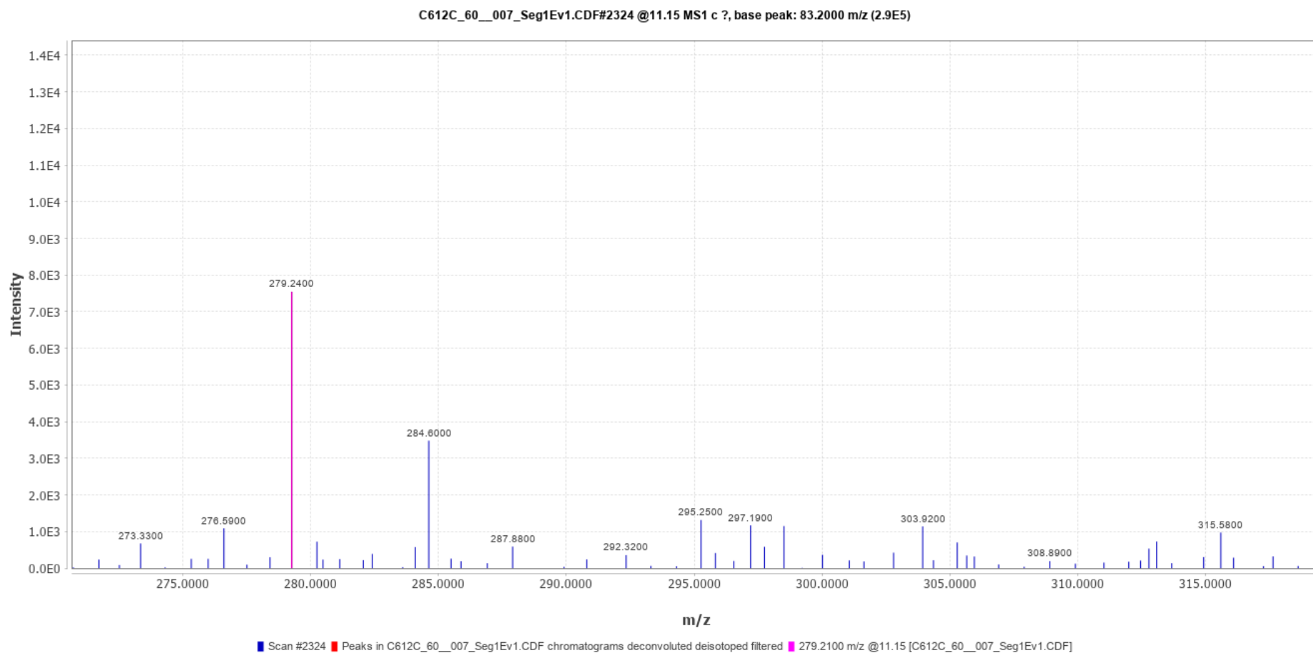
Spectrum No. 1
