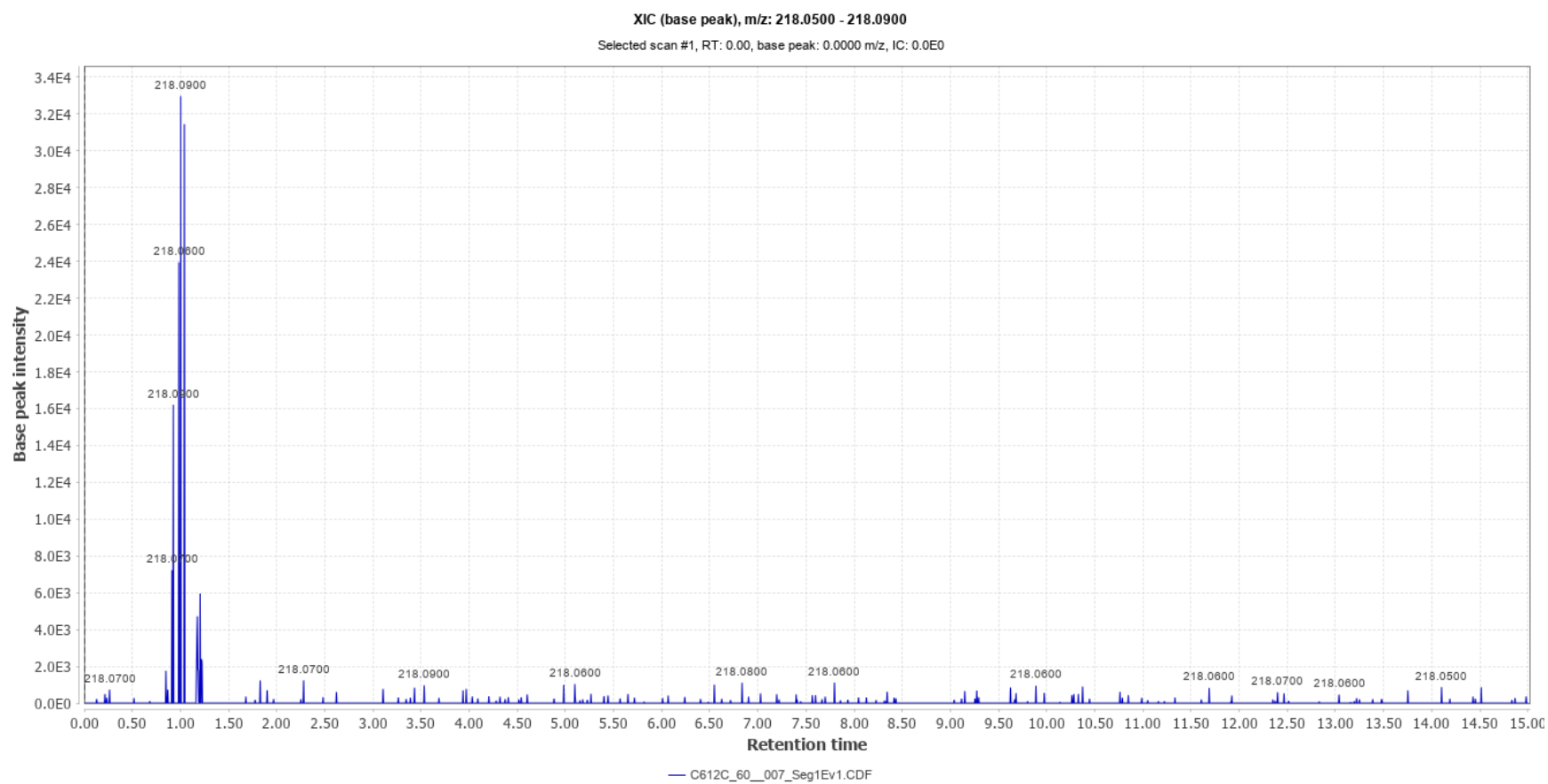
Chromatogram No. 2
