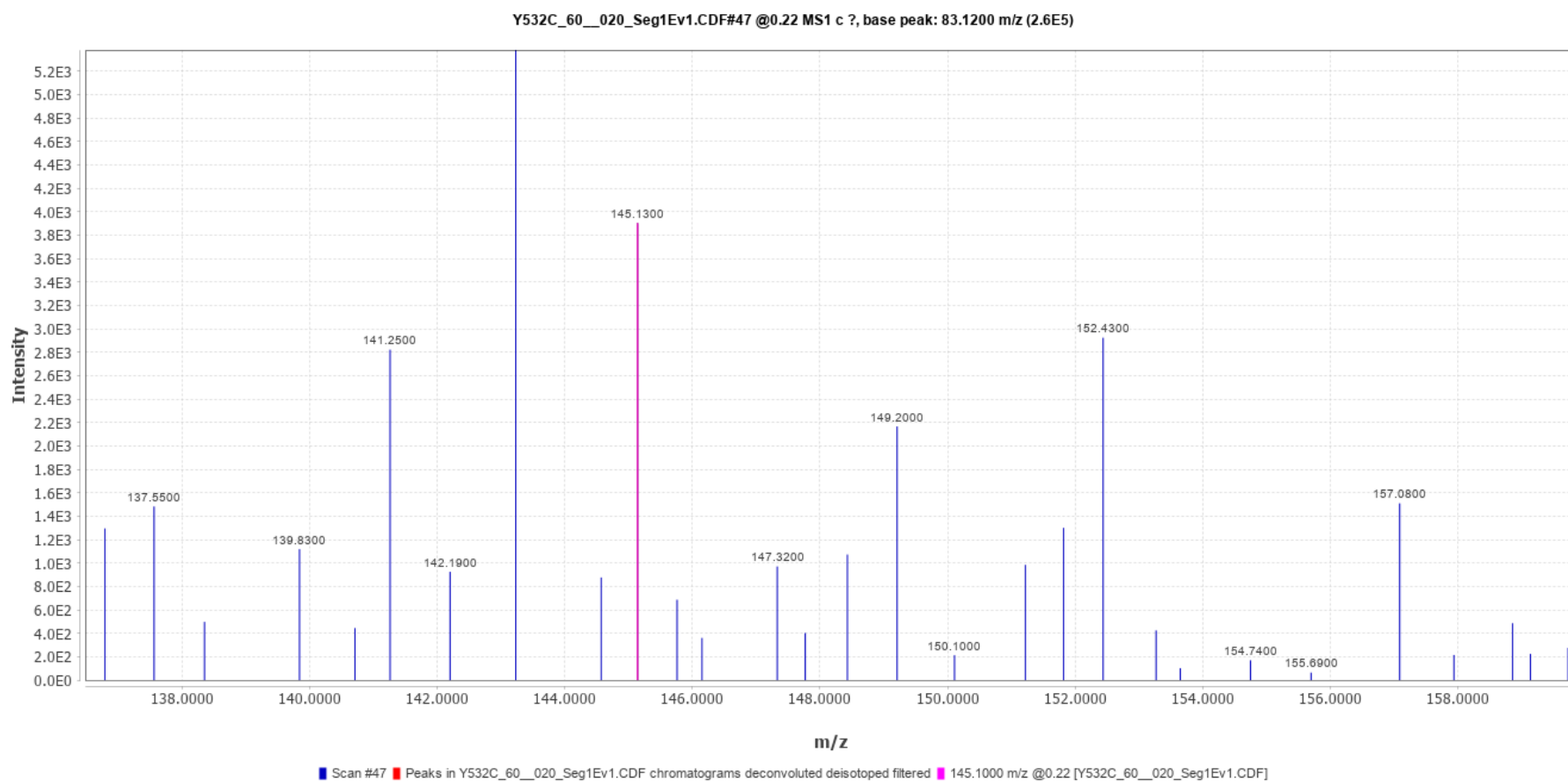
Spectrum No. 6
