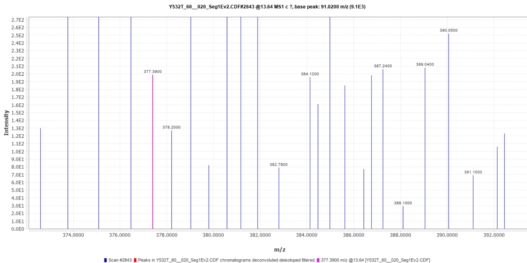
Spectrum No. 10
