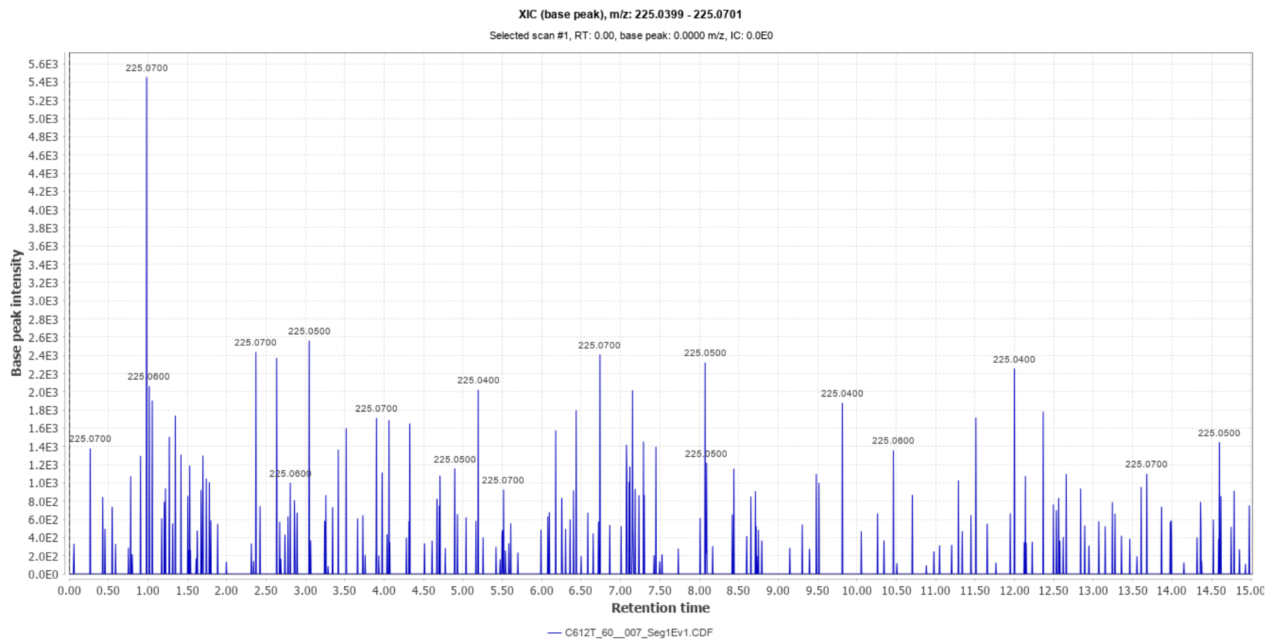
Chromatogram No. 8
