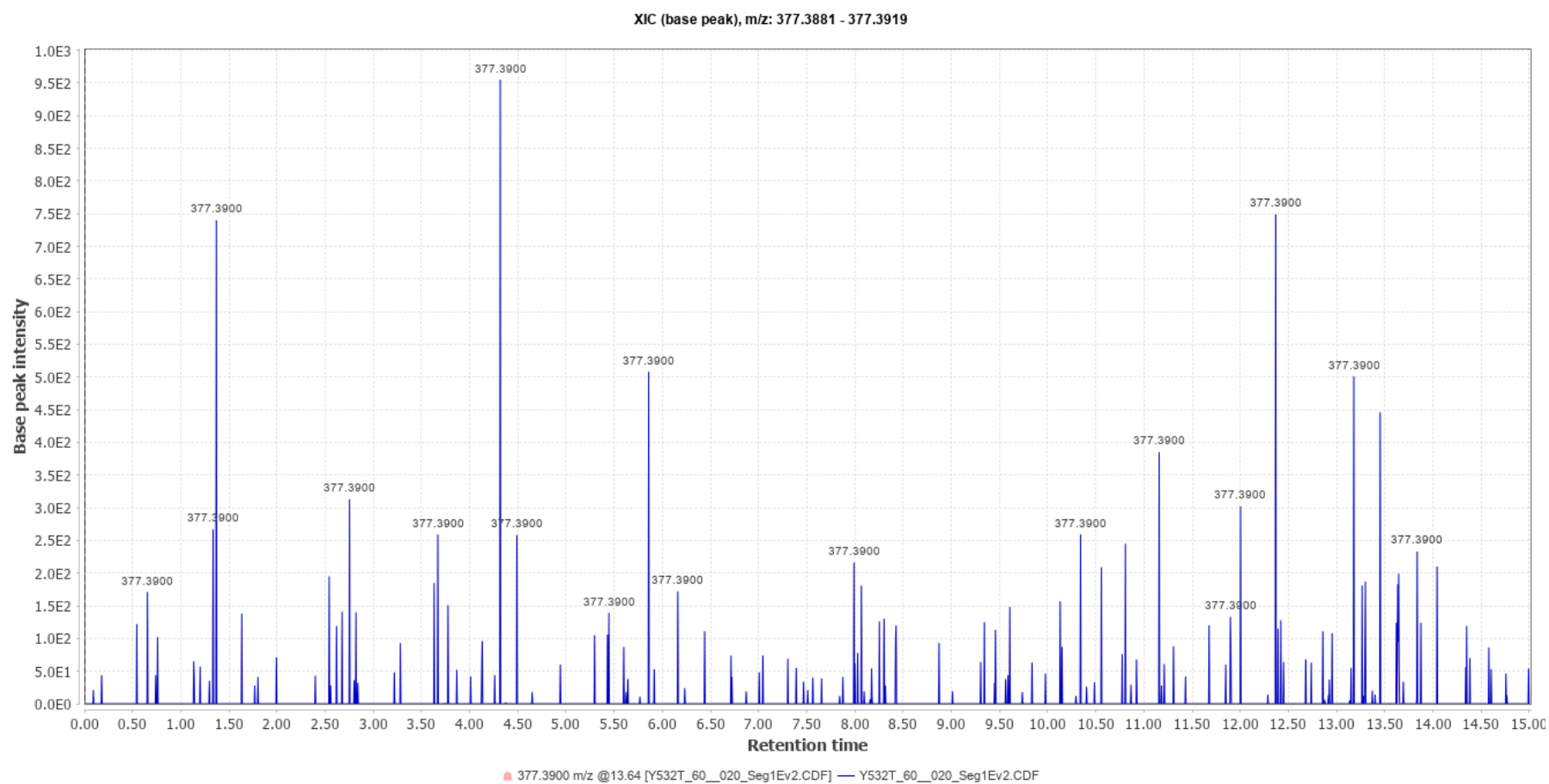
Chromatogram No. 10
