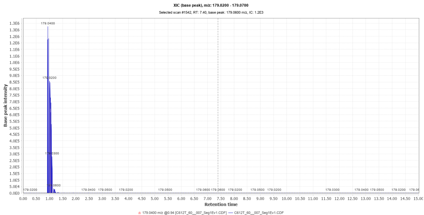
Chromatogram No. 9
