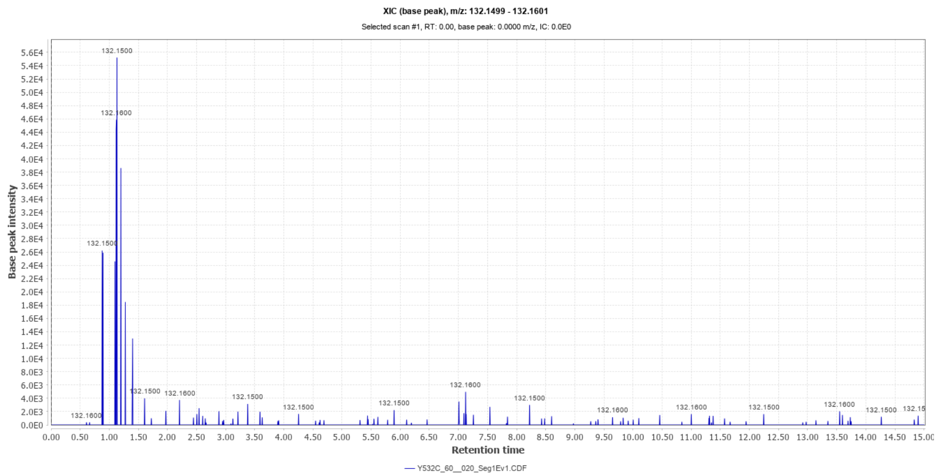
Chromatogram No. 5
