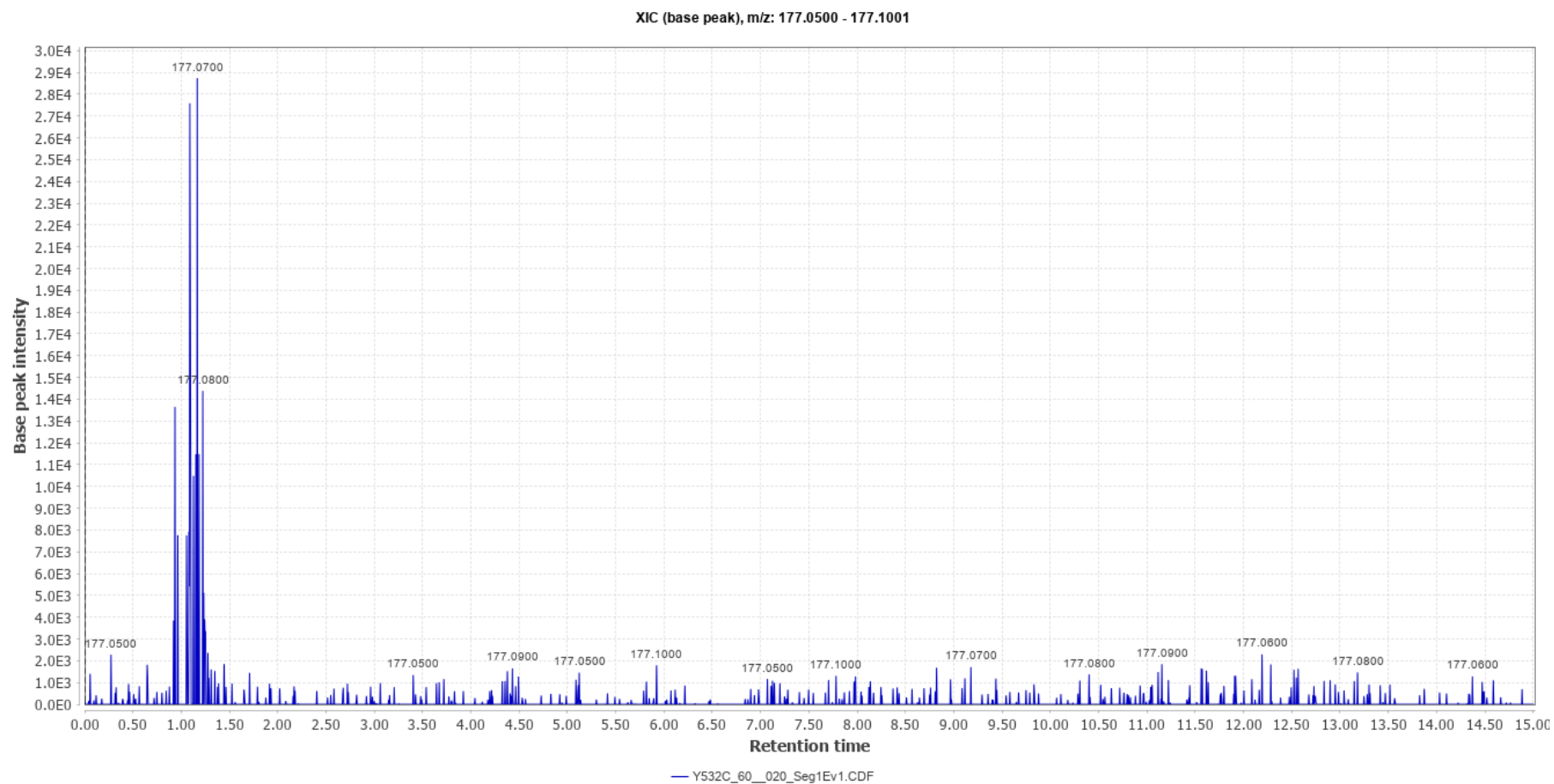
Chromatogram No. 4
