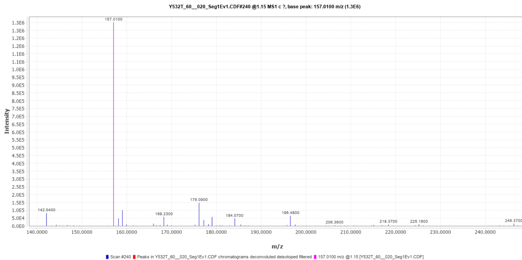
Spectrum No. 11
