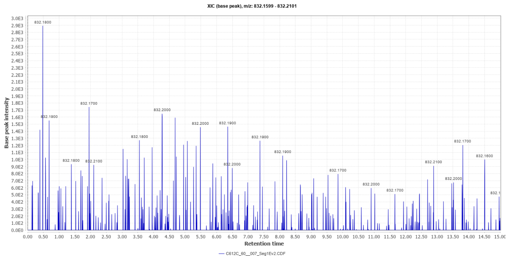
Chromatogram No. 3
