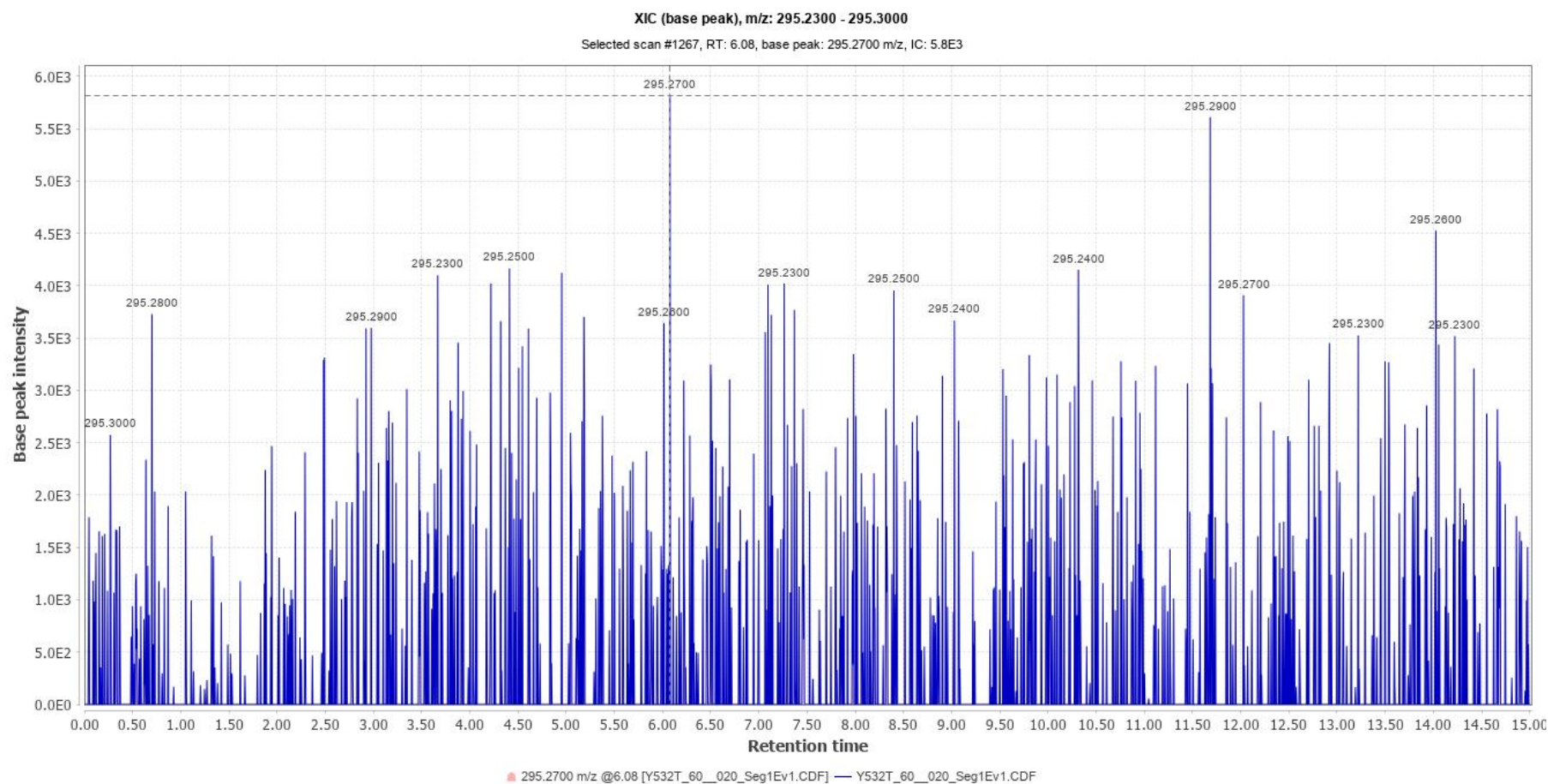
Chromatogram No. 12
