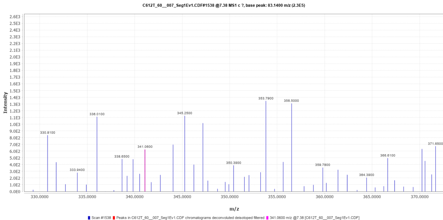
Spectrum No. 7
