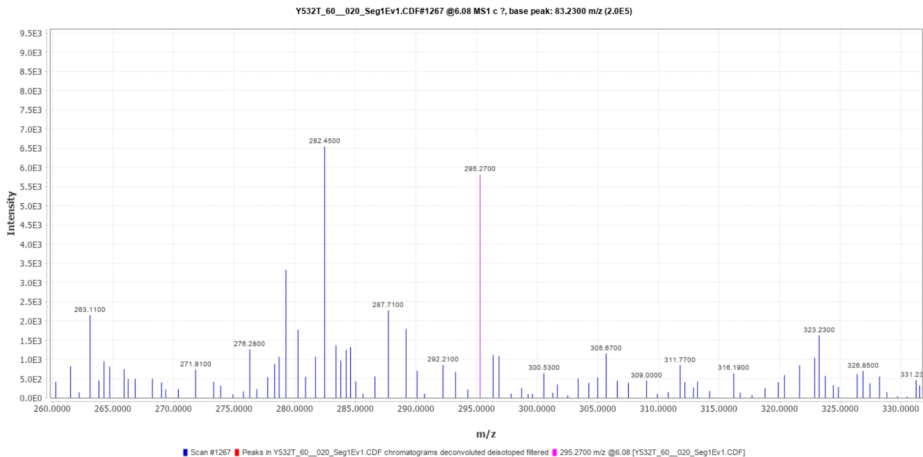
Spectrum No. 12
