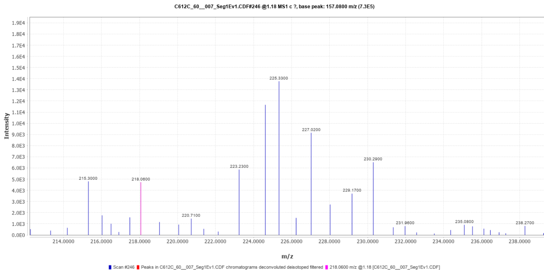
Spectrum No. 2
