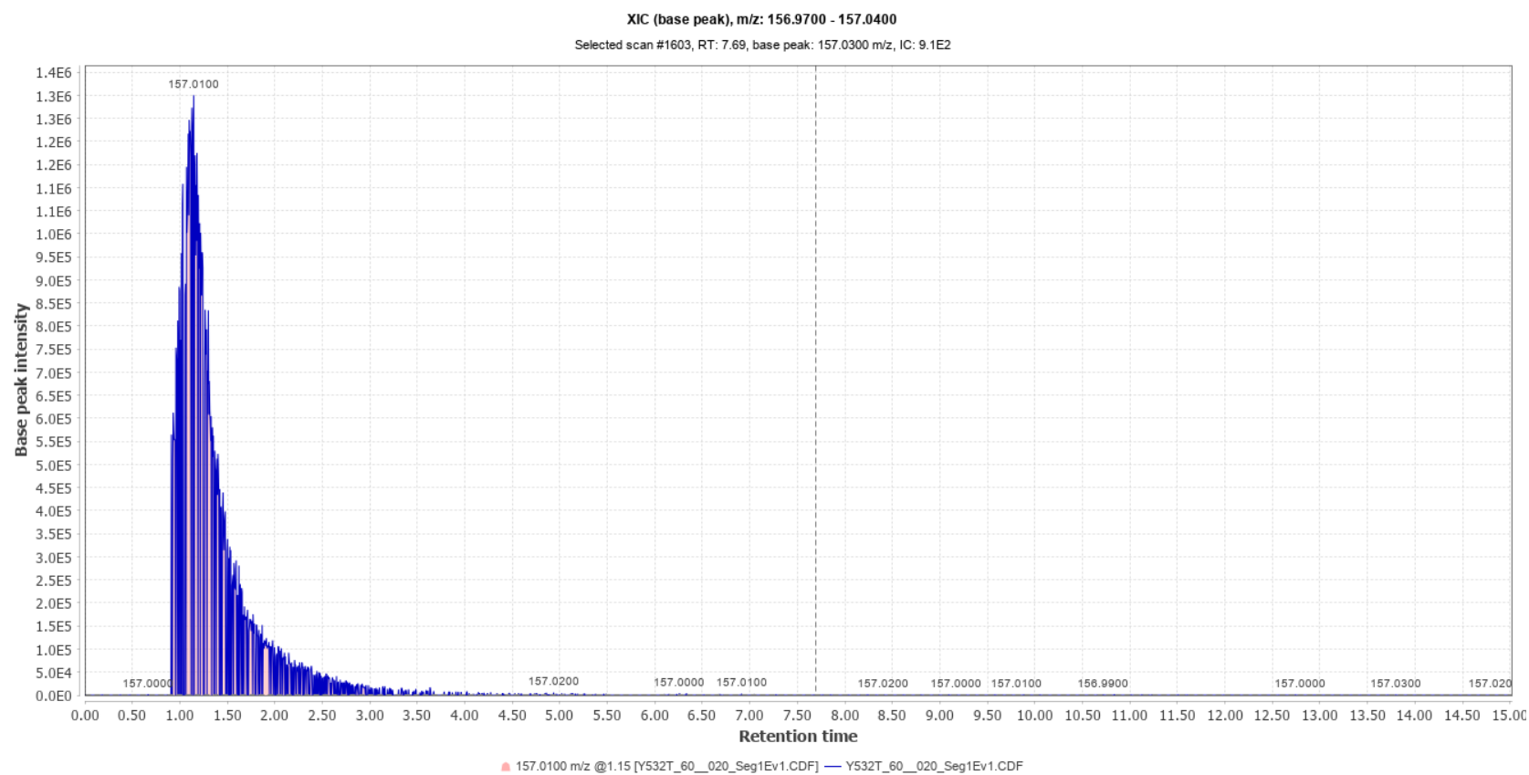
Chromatogram No. 11
