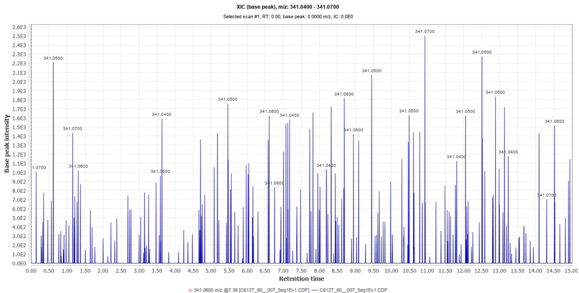
Chromatogram No. 7
