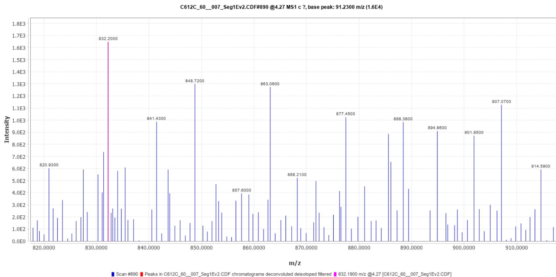
Spectrum No. 3
