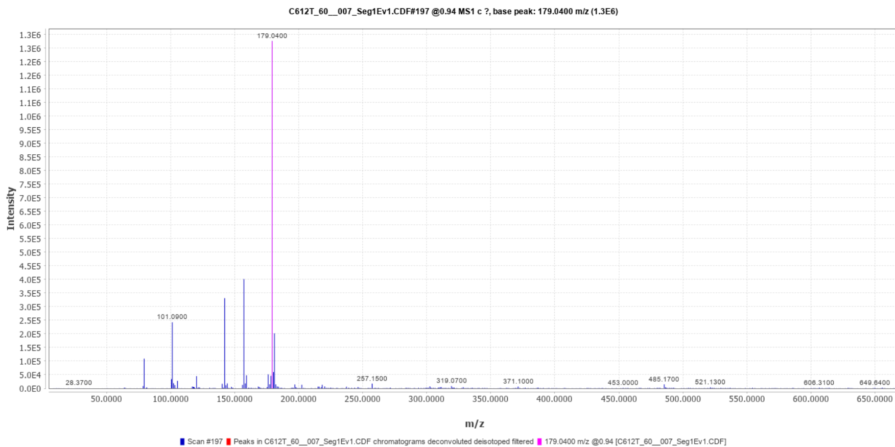
Spectrum No. 9
