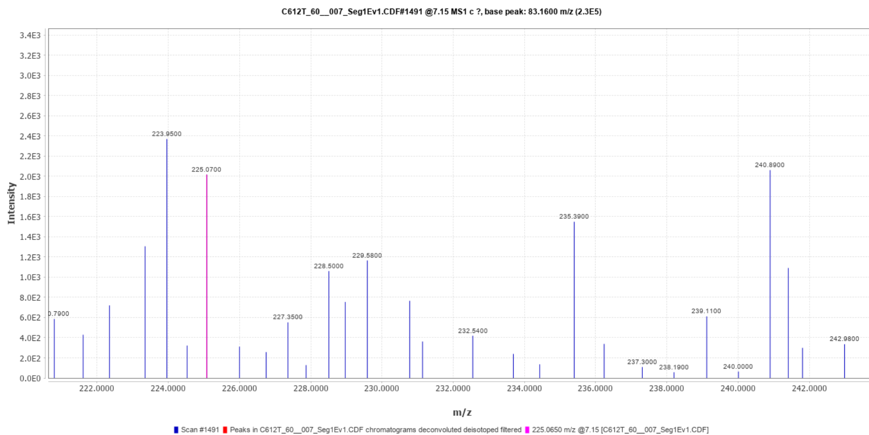
Spectrum No. 8
