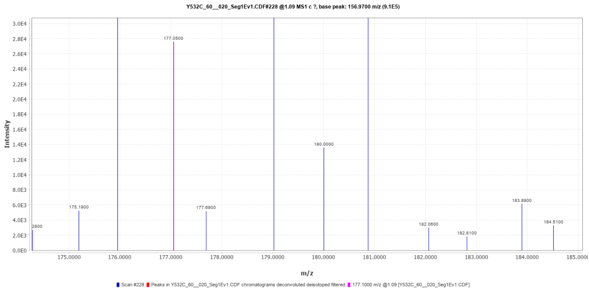
Spectrum No. 4
