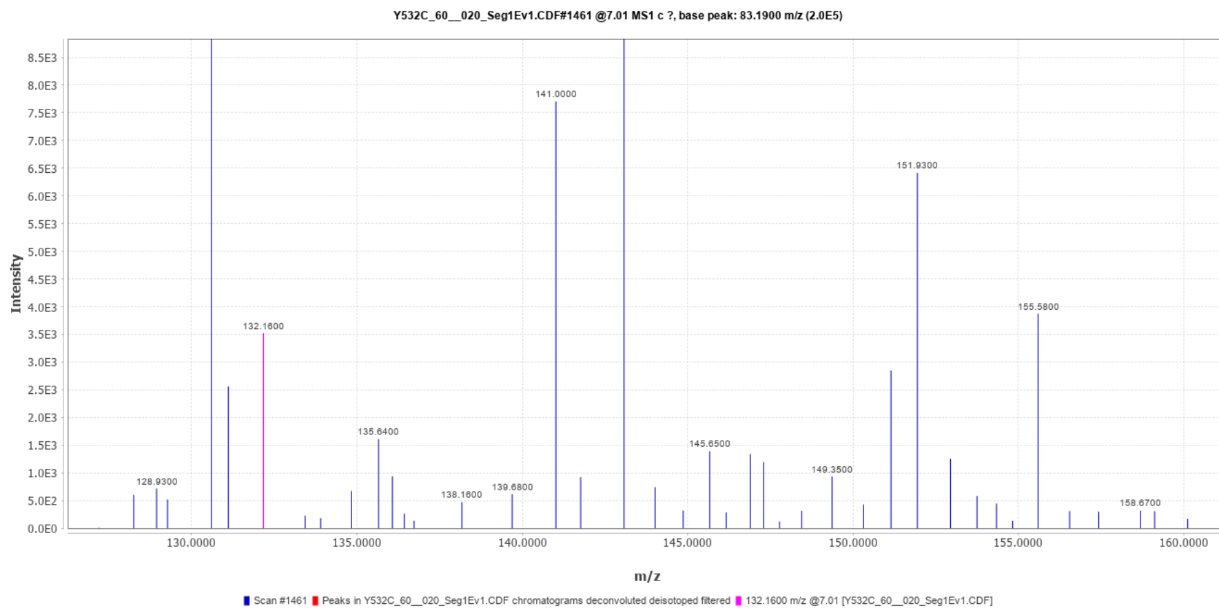
Spectrum No. 5
