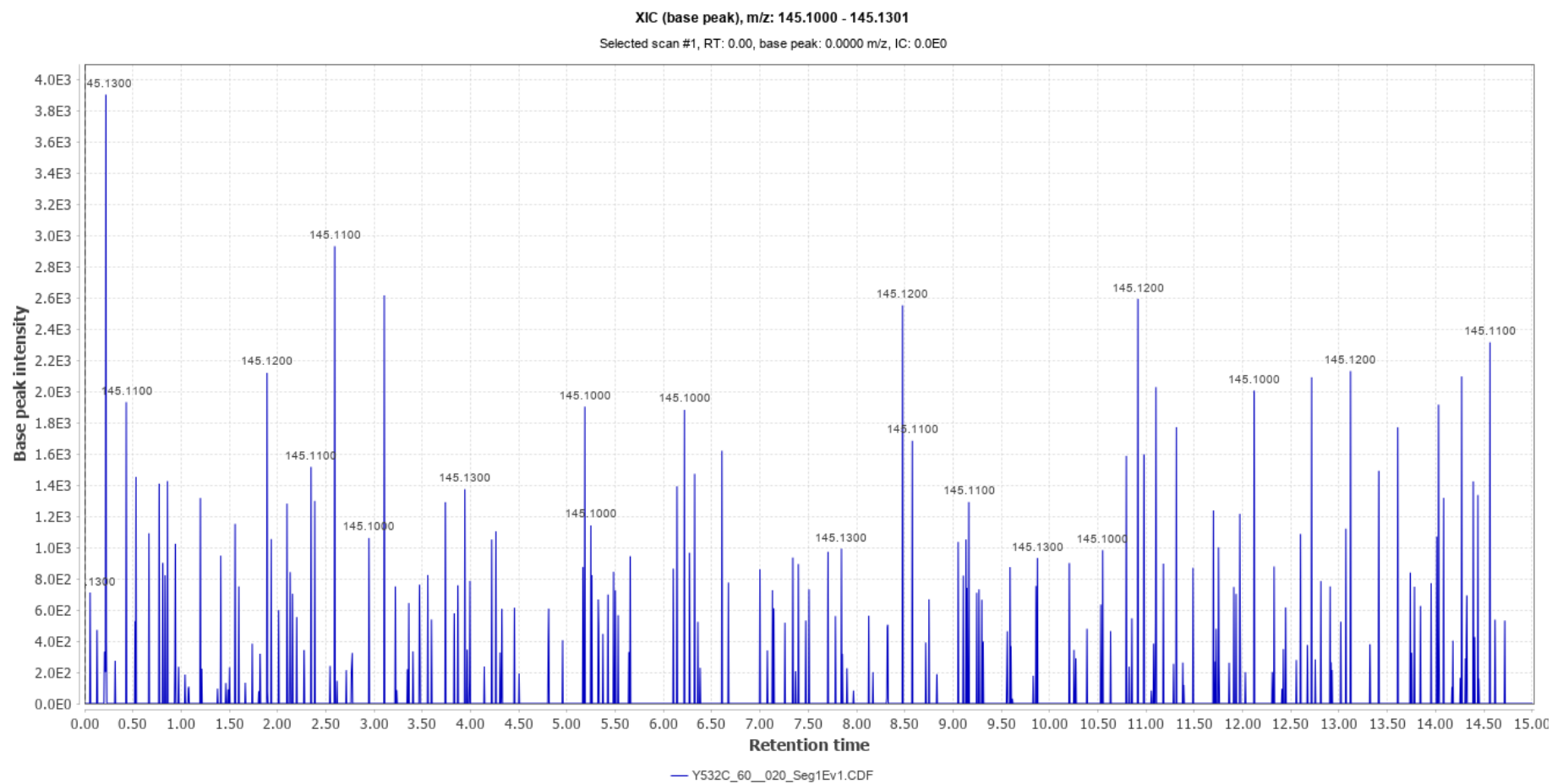
Chromatogram No. 6
