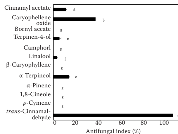
Figure 4. Antifungal activities of main constituents (200 µg per ml) of leaf oils from C. osmophloeum against P. noxius
