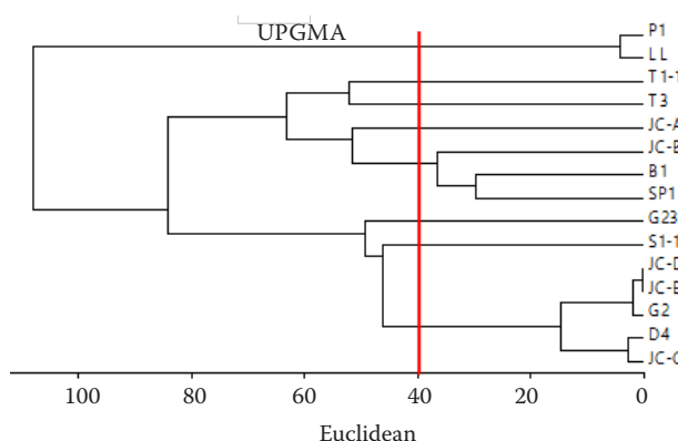
Figure 1. Dendrogram obtained by cluster analysis of the percentage composition of leaf oils from 15 provenances of C. osmophloeum
